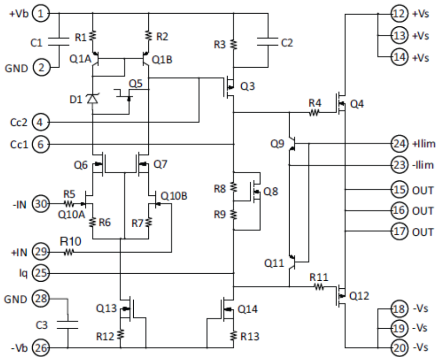
Figure 1: 等価回路図
