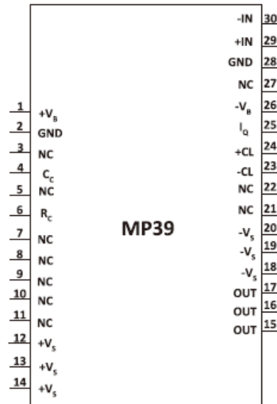
Figure 3: External Connections
