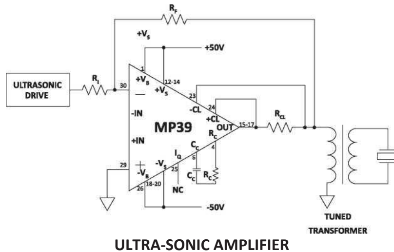
Figure 12: Typical Application
