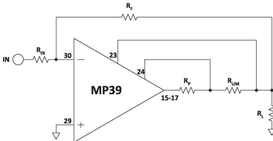
Figure 11: Current Limit
