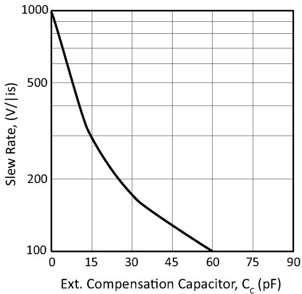
Figure 10: Slew Rate
