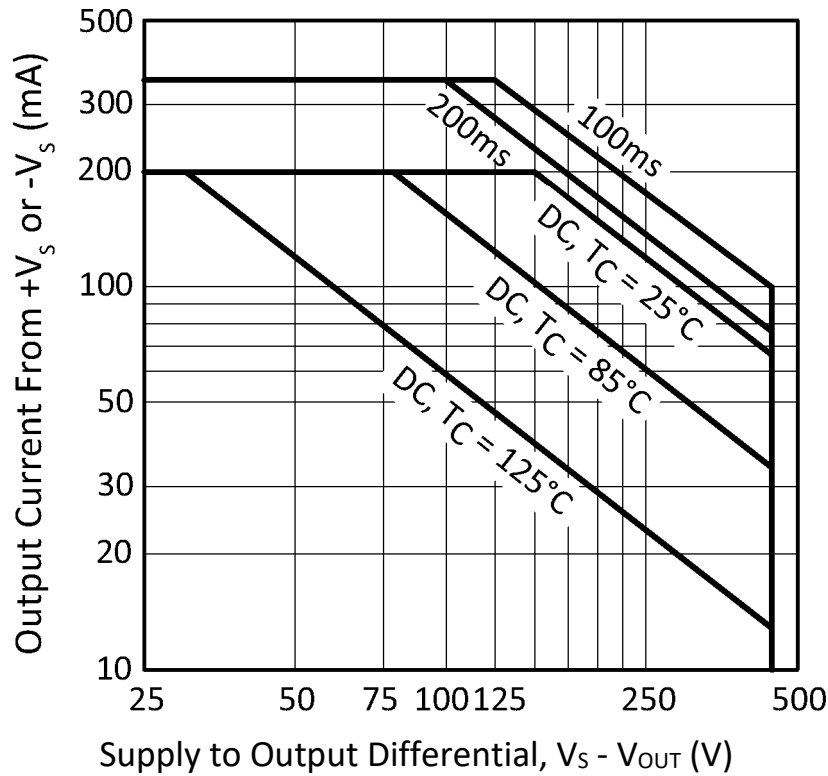
Figure 16: SOA
