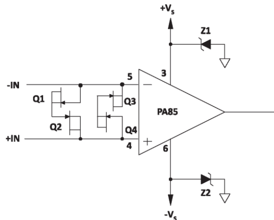
Figure 18: 過電圧保護
