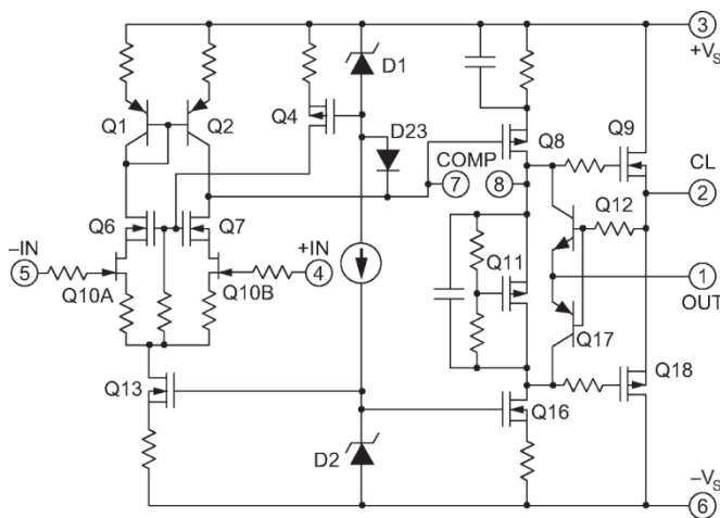
Figure 1: 等価回路図
