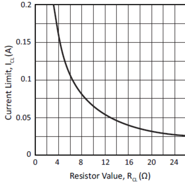
Figure 13: Current Limit
