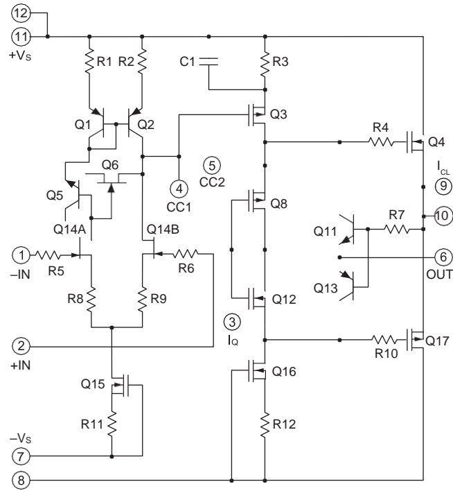
Figure 1: 等価回路図
