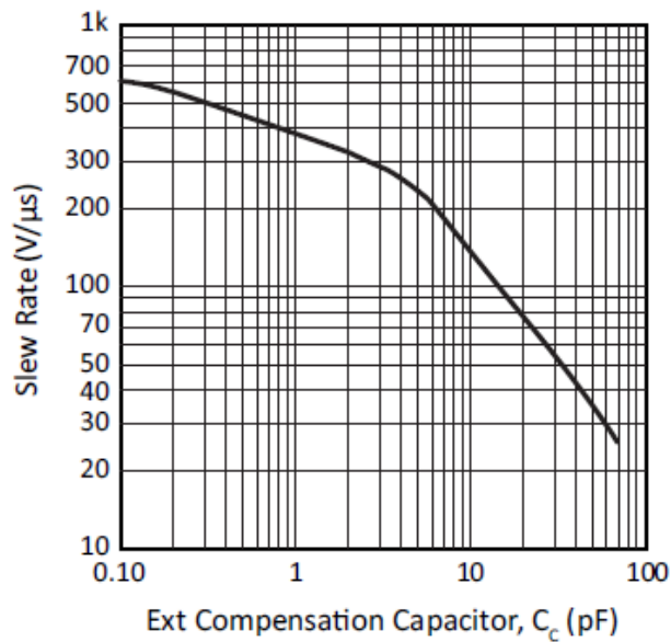
Figure 10: Slew Rate
