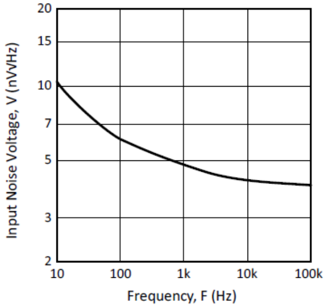
Figure 12: Input Noise Voltage
