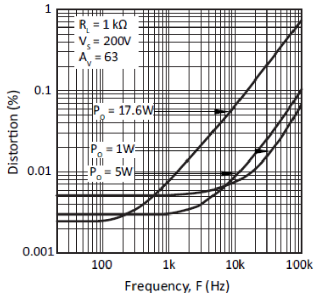
Figure 11: Harmonic Distortion
