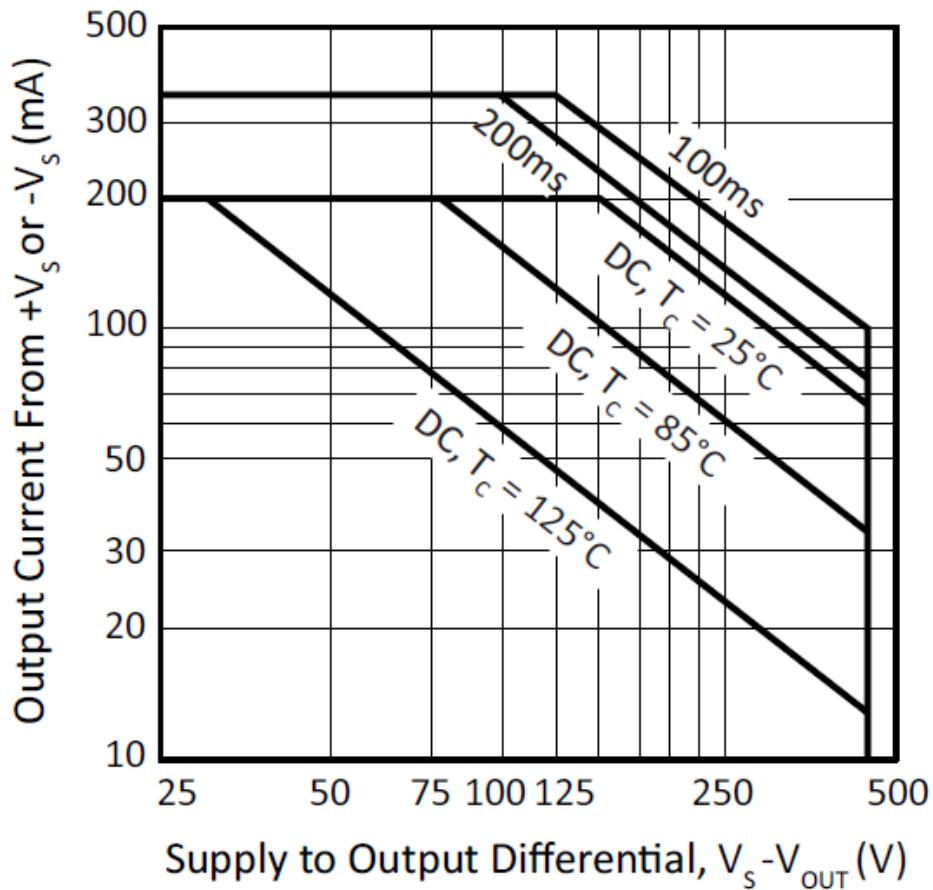
Figure 15: SOA
