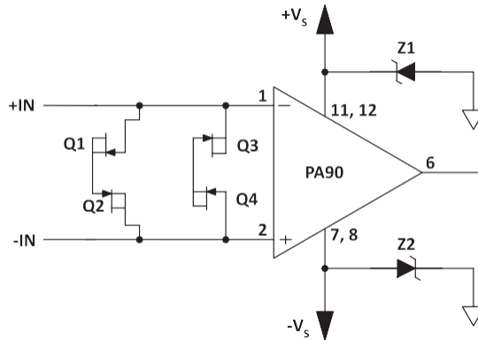
Figure 17: 過電圧保護
