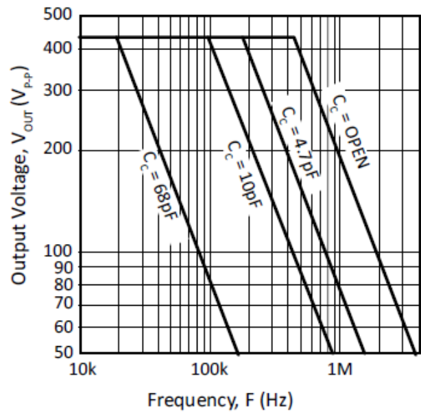
Figure 9: Power Response
