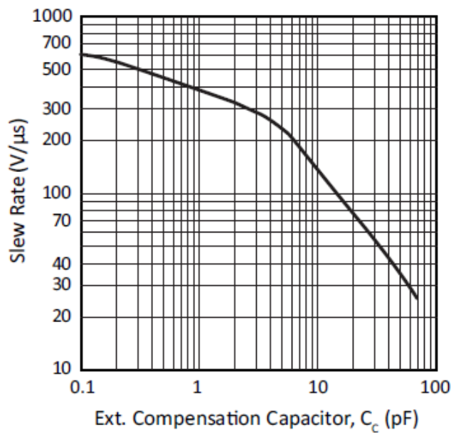
Figure 10: Slew Rate
