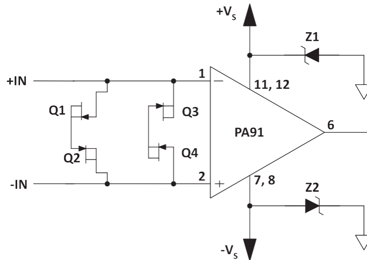
Figure 16: Overvoltage Protection
