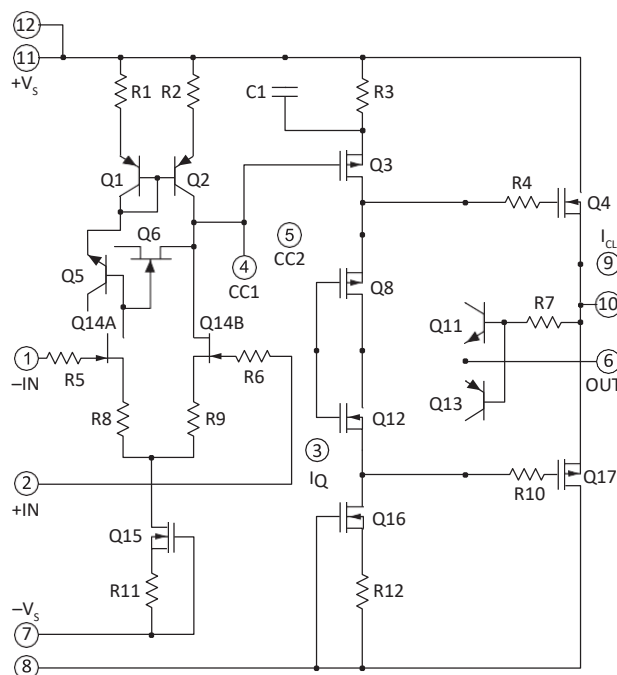
Figure 1: 等価回路図
