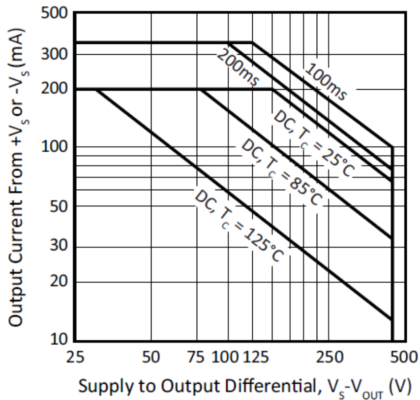
Figure 14: SOA
