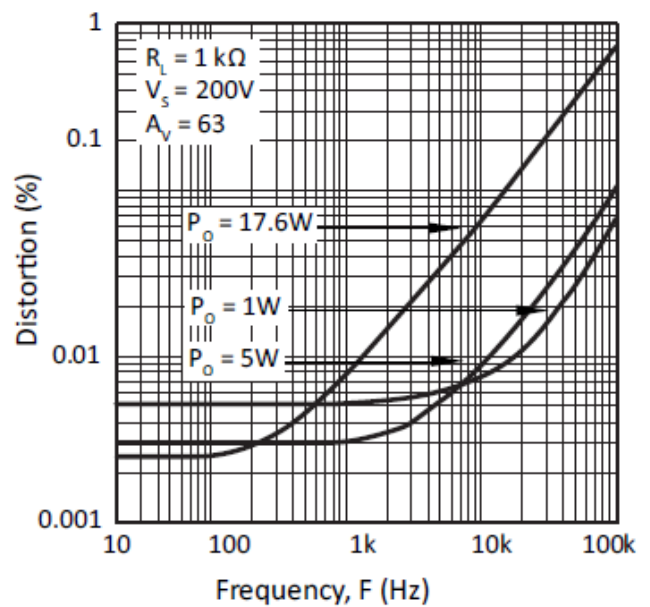
Figure 11: Harmonic Distortion
