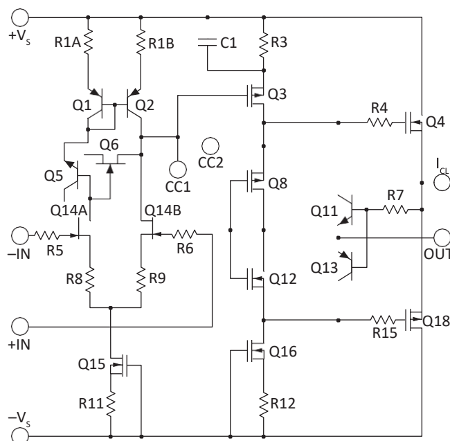
Figure 1: 等価回路図
