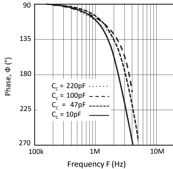
Figure 7: Phase Response
