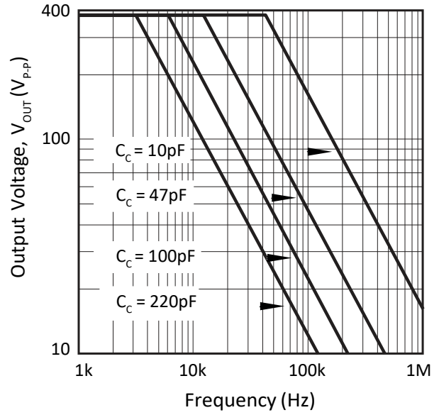
Figure 9: Power Response
