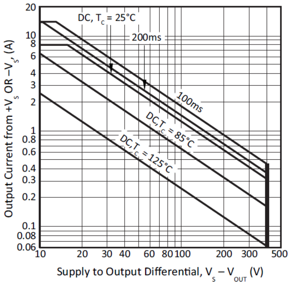
Figure 14: SOA
