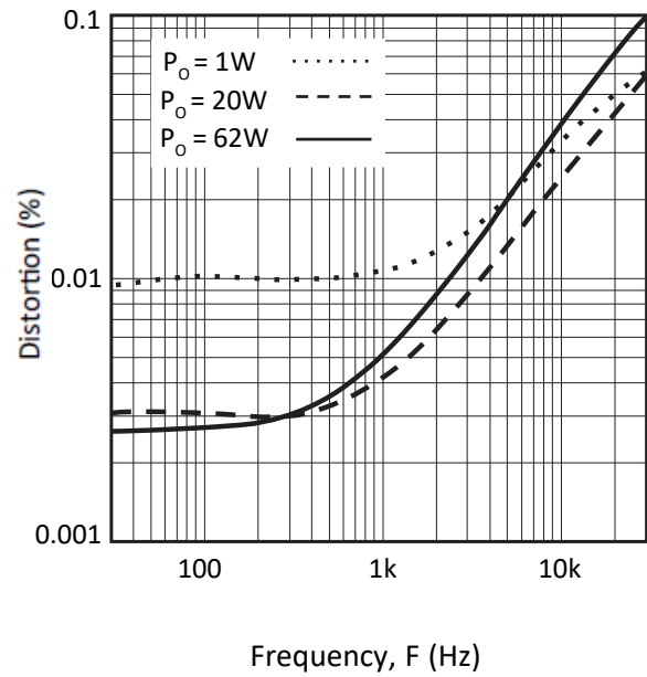
Figure 11: Harmonic Distortion
