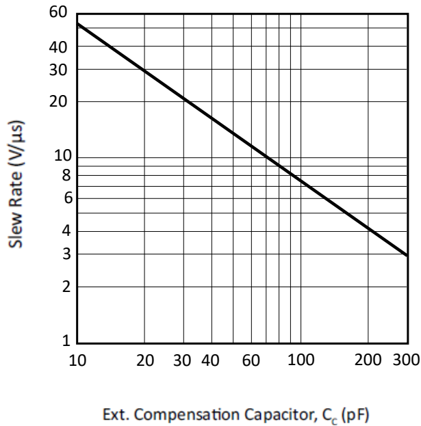
Figure 10: Slew Rate
