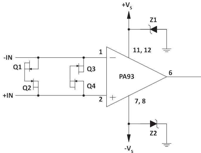
Figure 16: 過電圧保護
