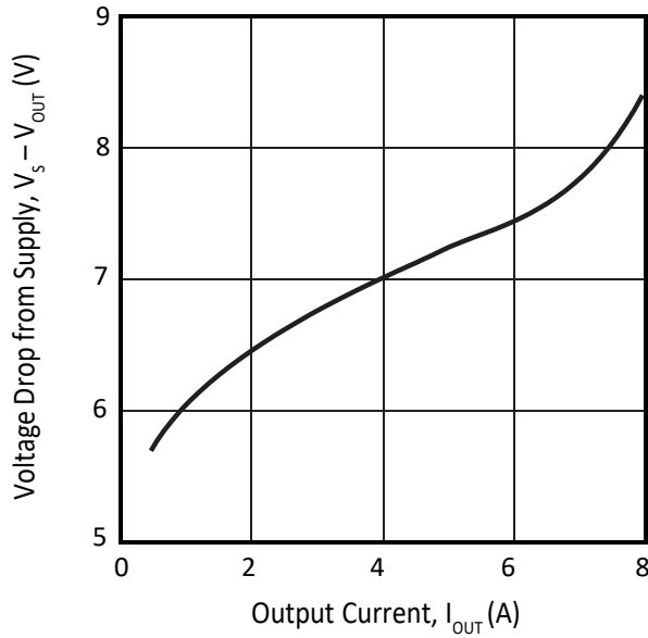
Figure 8: Output Voltage Swing
