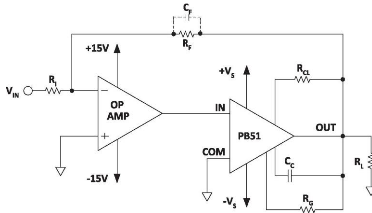
Figure 16: Typical Application
