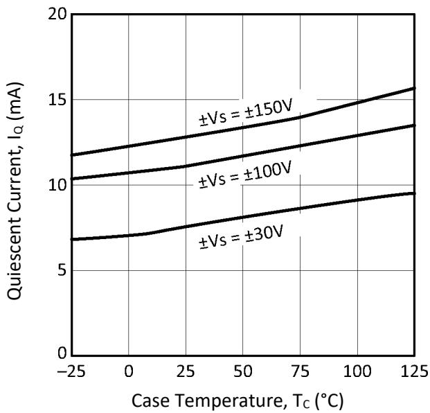
Figure 9: Quiescent Current
